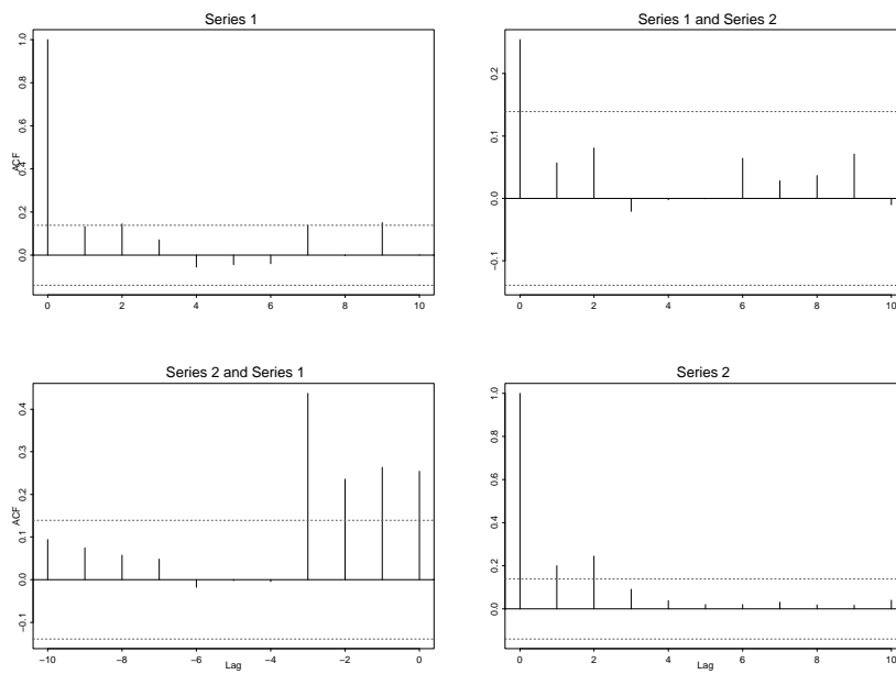
Figure 5: ACF, Squared VAR(1) Residuals
