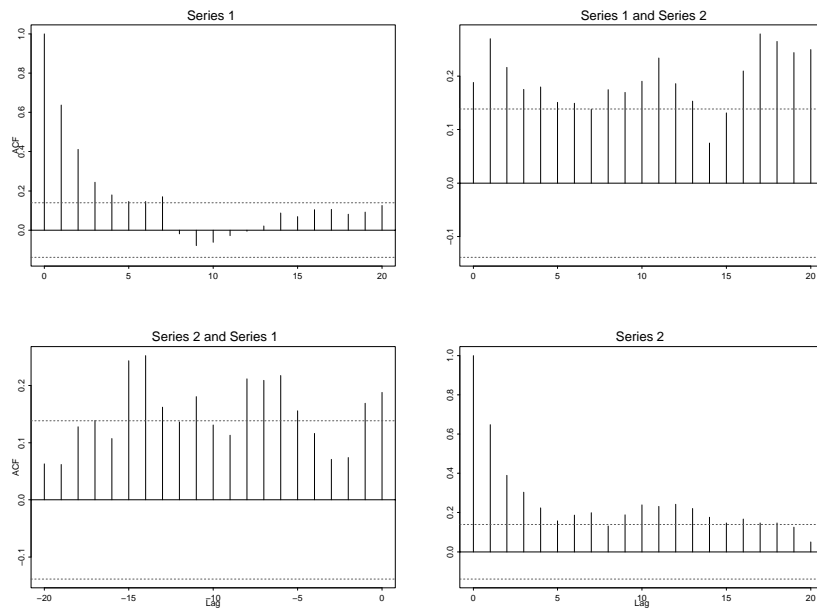
Figure 2: ACF, Squared Detrended Data
