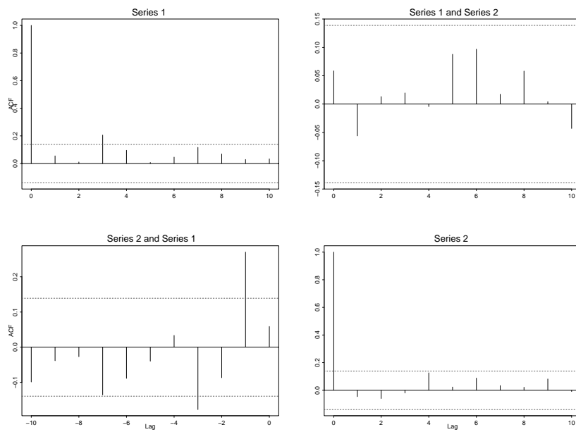
Figure 4: ACF, VAR(1) Residuals
