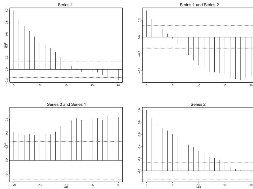
Figure 1: ACF, Detrended Data
